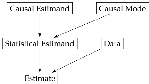
Figure 4.1: The Identification-Estimation Flowchart – a flowchart that illustrates the process of moving from a target causal estimand to a corresponding estimate, through identification and estimation. In contrast to Figure 2.5, this version is augmented with a causal model and data.
